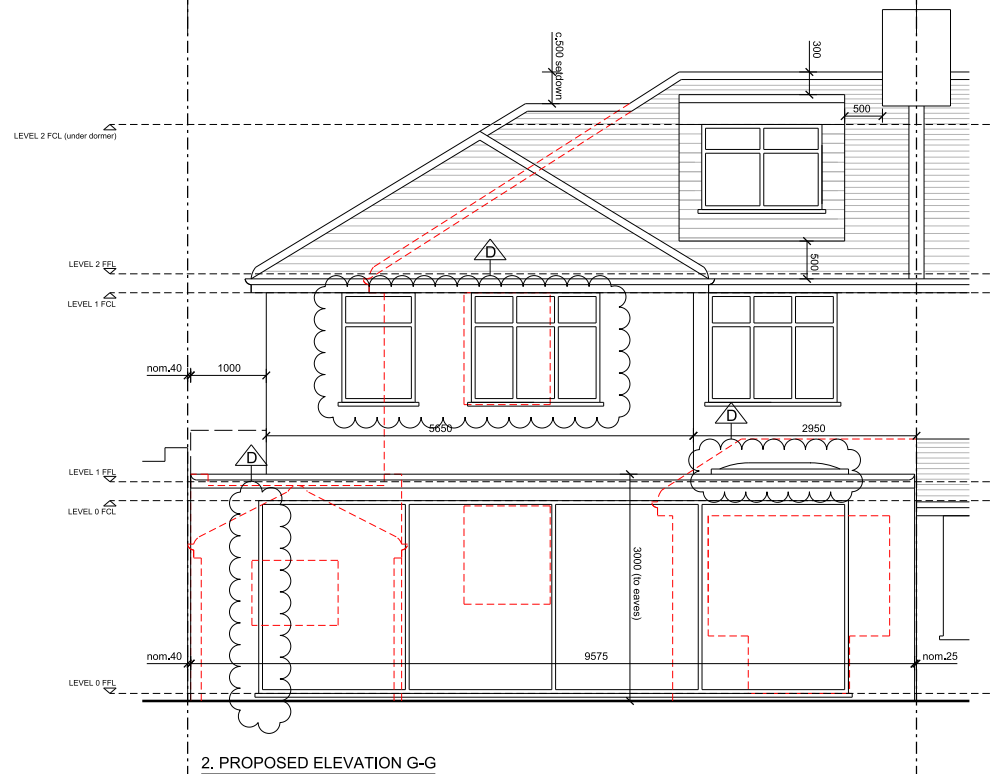
2. PROPOSED ELEVATION G-G
