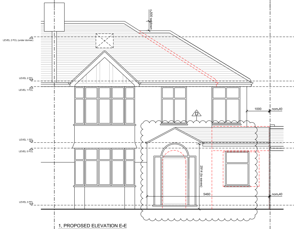
1. PROPOSED ELEVATION E-E
