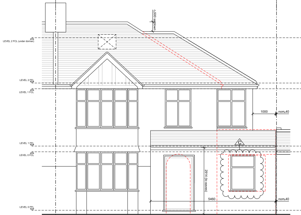
1. PROPOSED ELEVATION E-E
