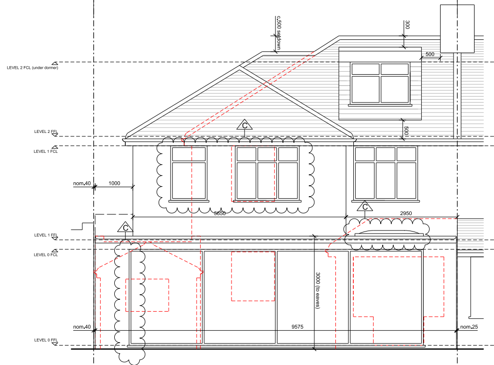
2. PROPOSED ELEVATION G-G
