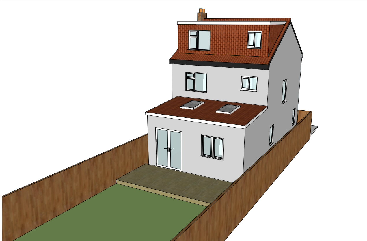
Proposed Rear/Side 3D view
