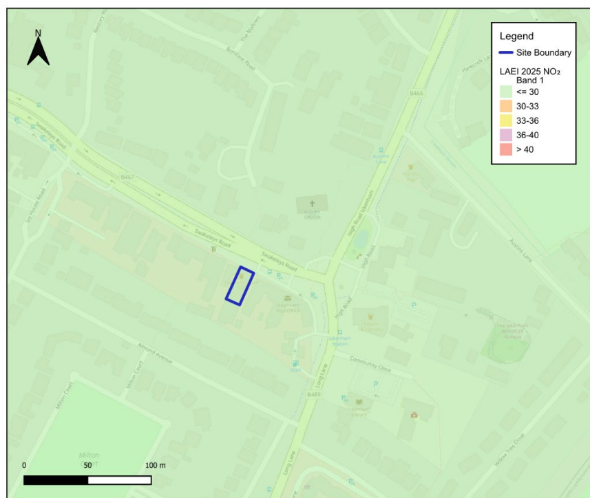
Figure 7: LAEI NO 2 annual mean predicted concentrations for 2025 ( \mu\text{g}/\text{m}^3 )
