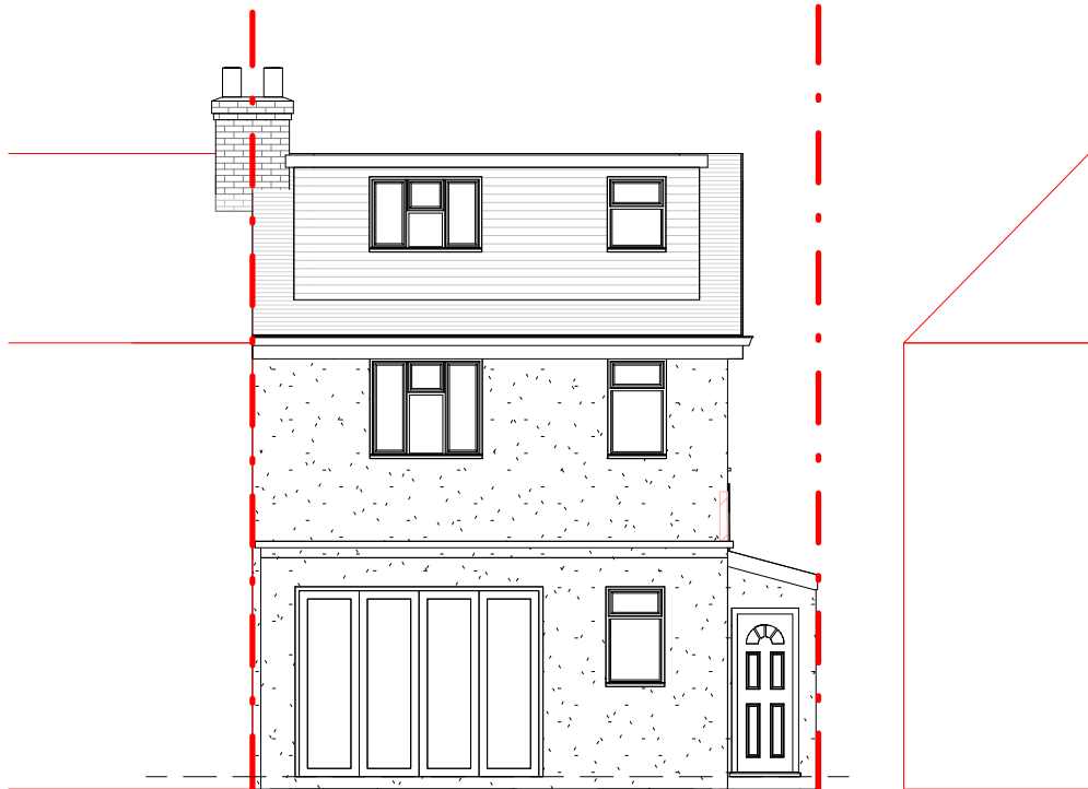
AE-0030-01 - Rear Elevation
