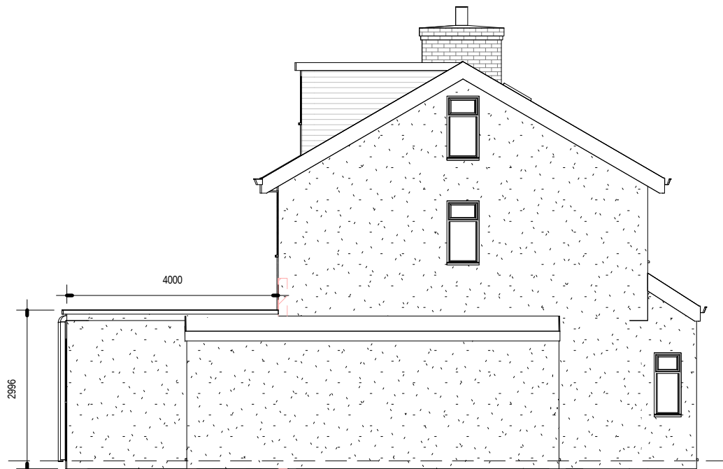
AE-0040-01 - Side Elevation
