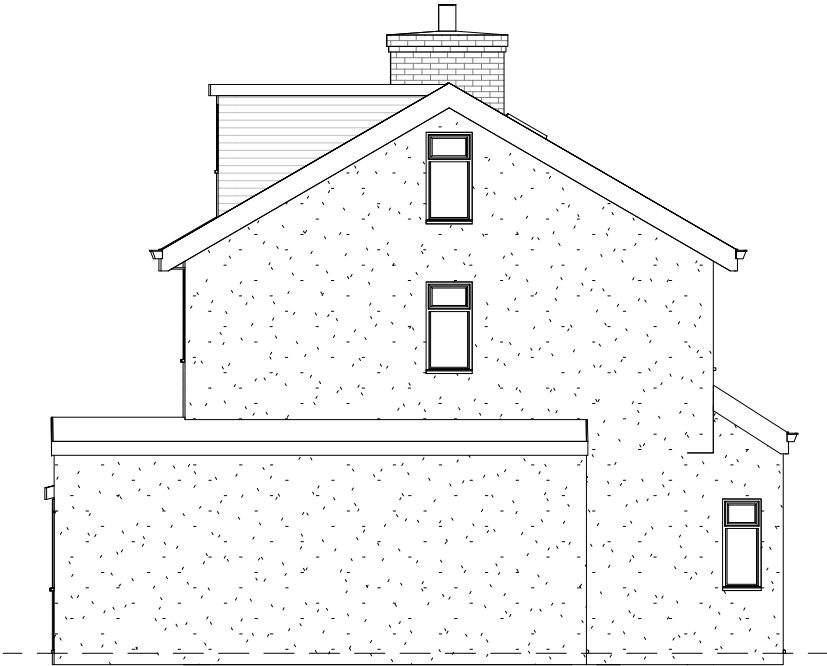
AE-0040-01 - Side Elevation
