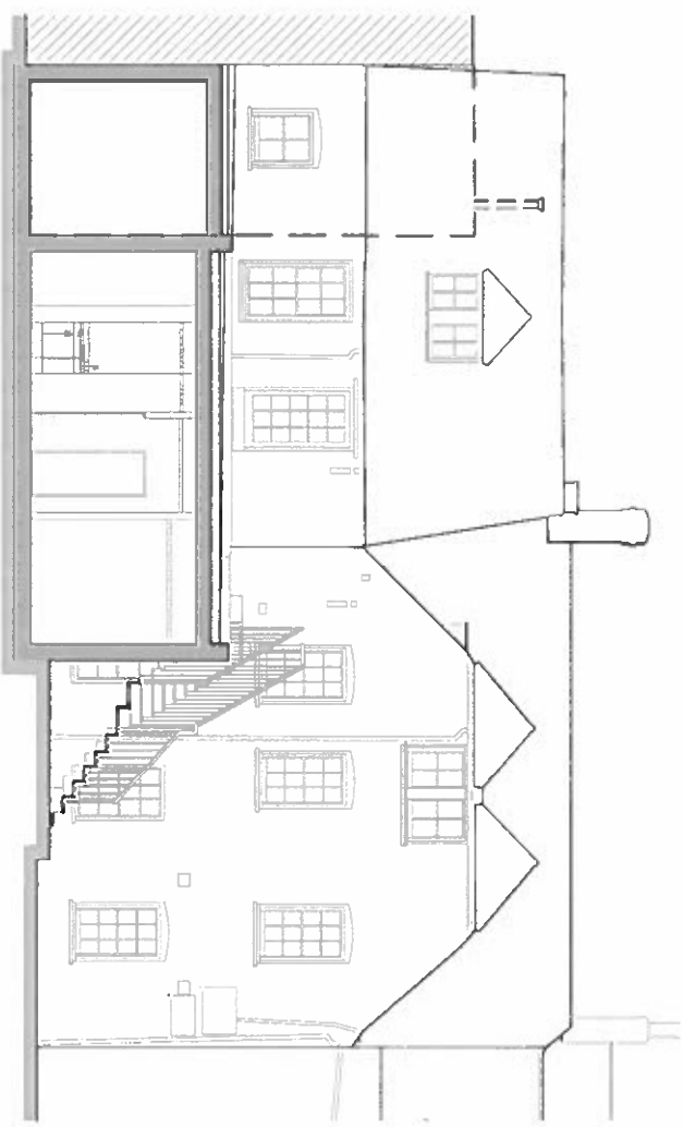
Rear Elevation 1:100
