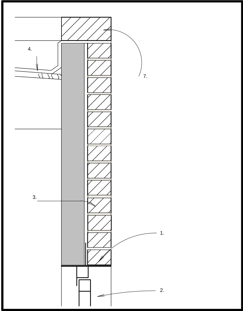
Cross section bike store - door
