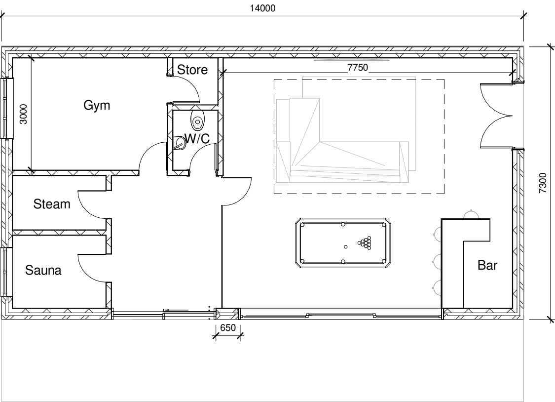
00 - Proposed Plan 1 : 100
