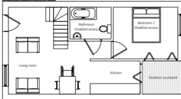
GROUND FLOOR PLAN @ 1:50
