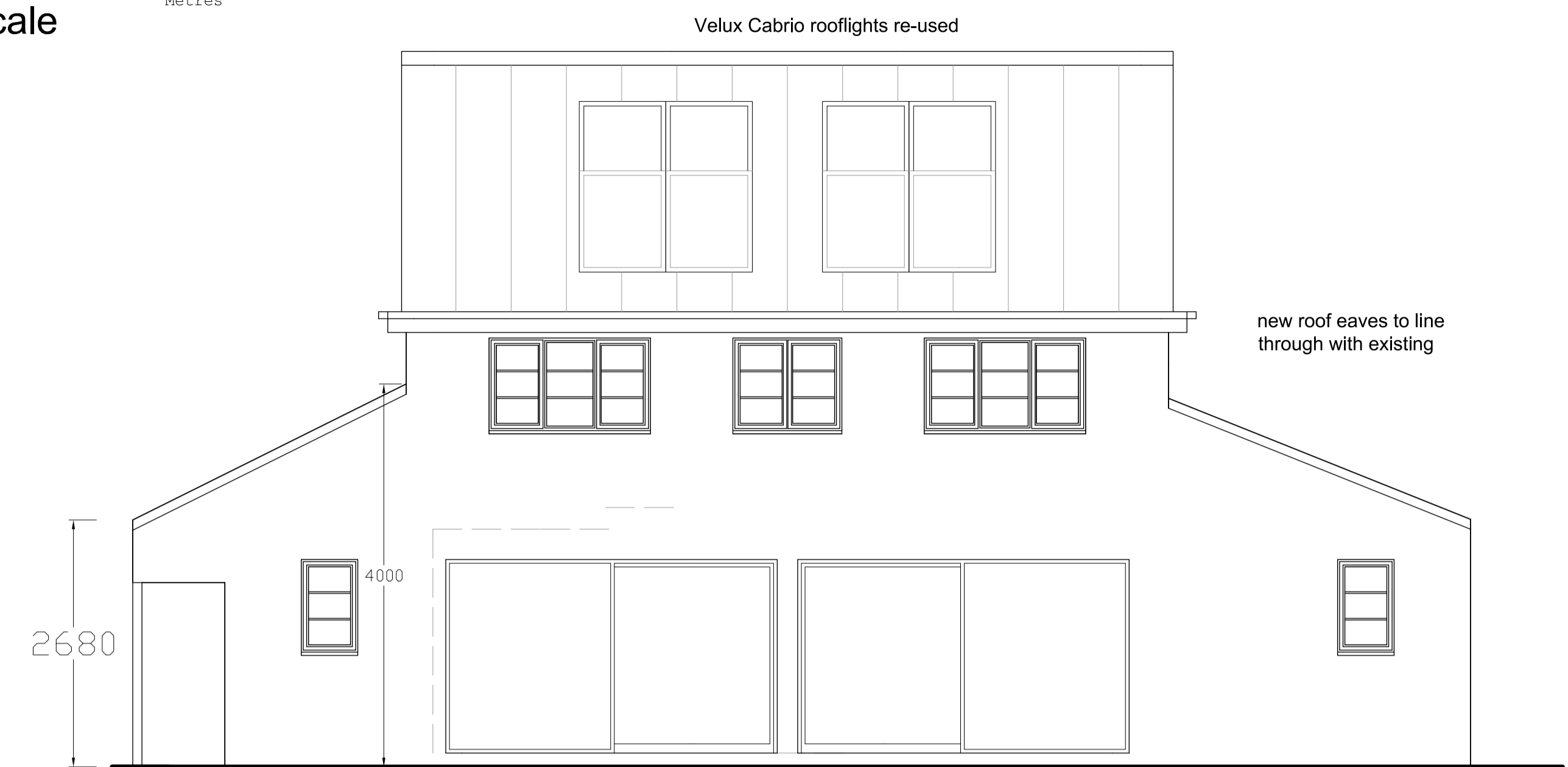
REAR ELEVATION
