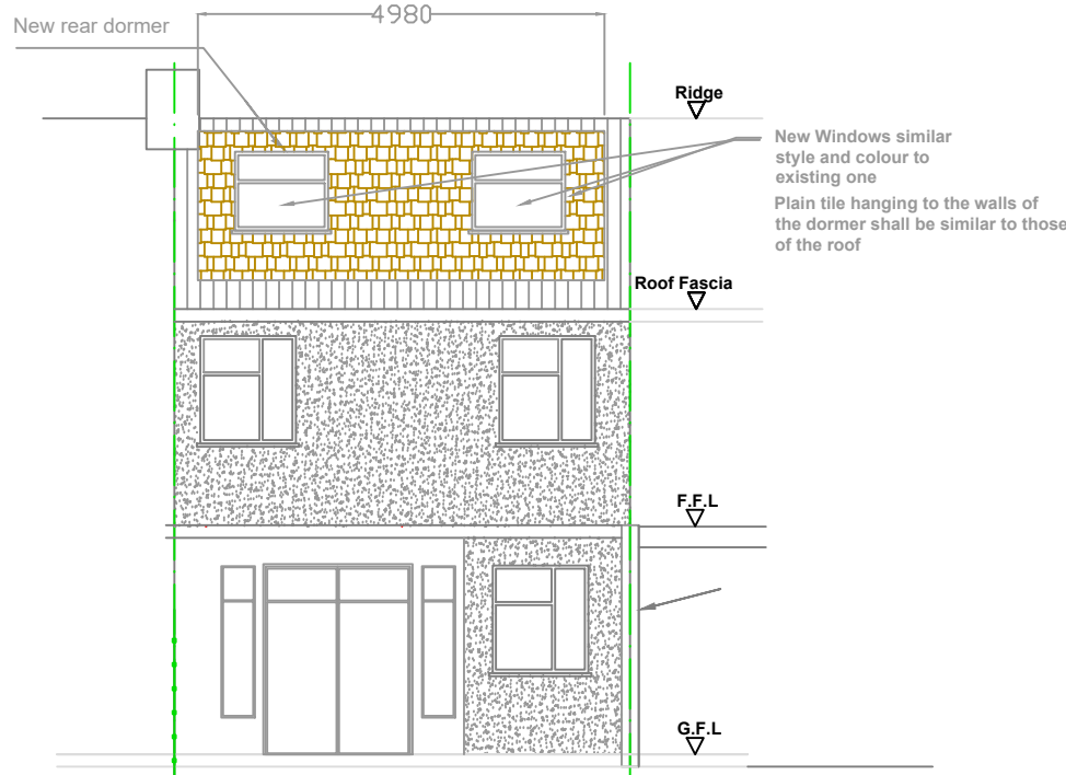
REAR ELEVATION
