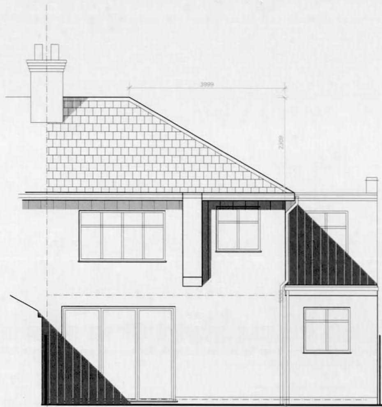
Rear (South) Elevation
