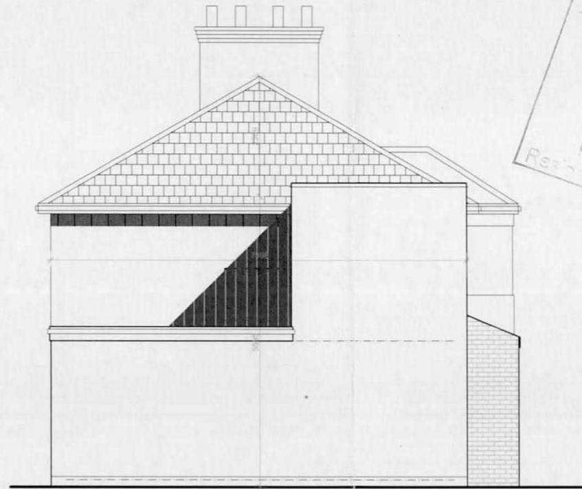
Side (East) Elevation
