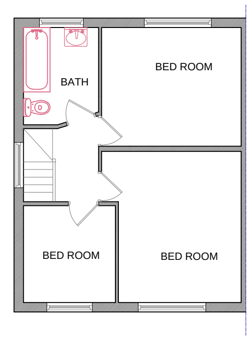
EXISTING/PROPOSED FIRST FLOOR PLAN Scale 1:100
