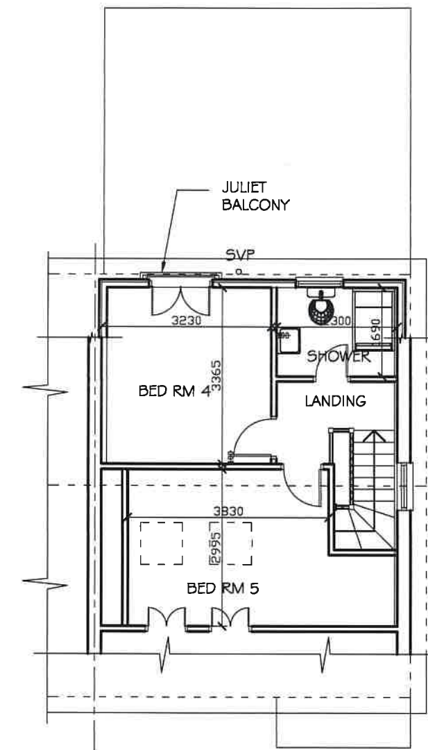
PROPOSED LOFT FLOOR PLAN SCALE= 1:100
