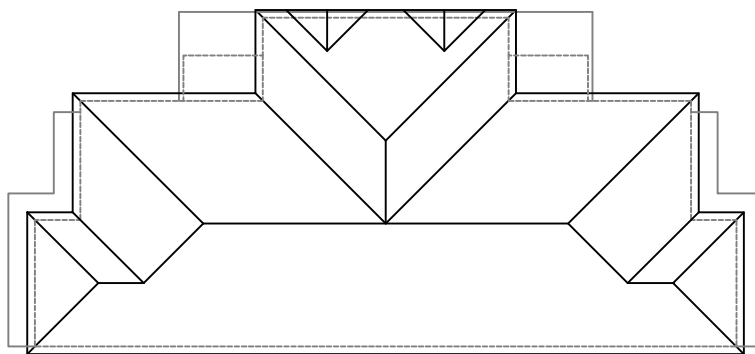
ROOF PLAN
