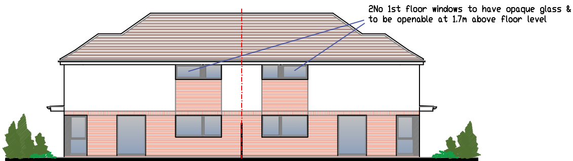
REAR ELEVATION
