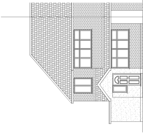
Existing Front Elevation Scale 1:100
