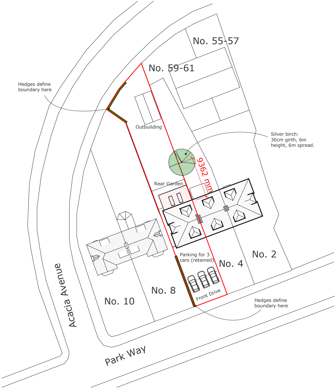
Block Plan
