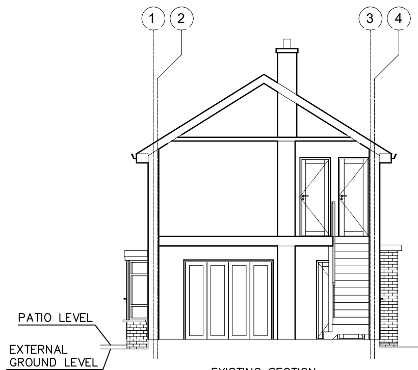
EXISTING SECTION
