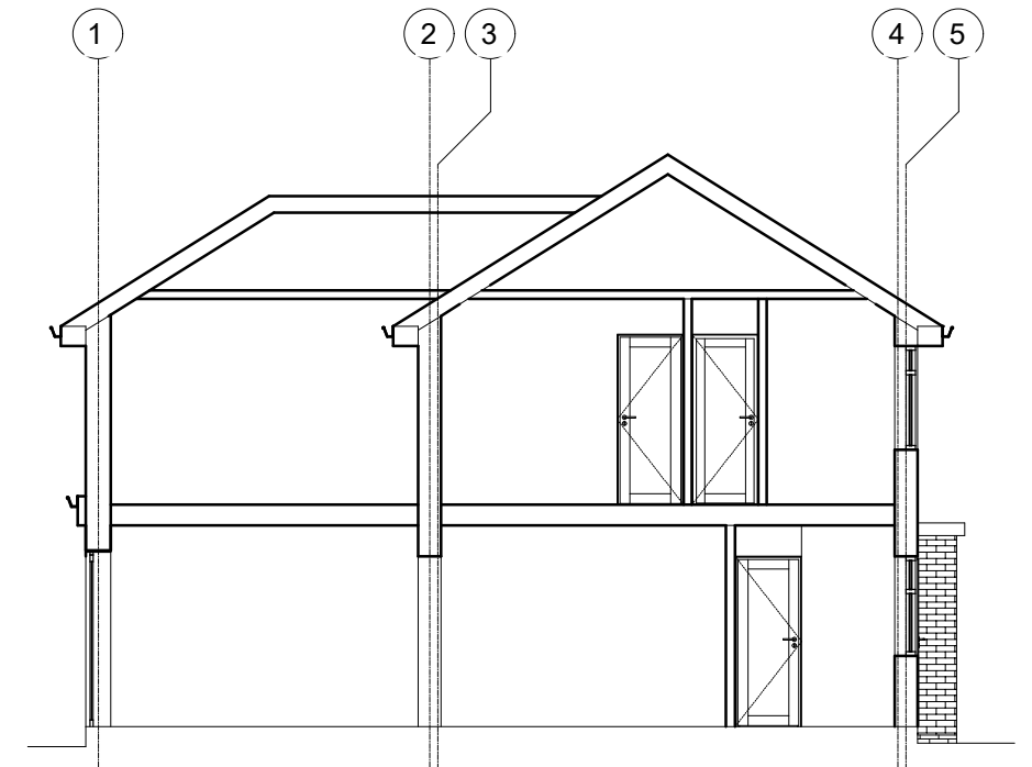
PROPOSED SECTION
