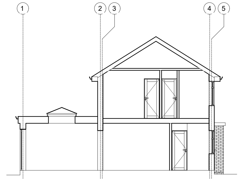
EXISTING SECTION
