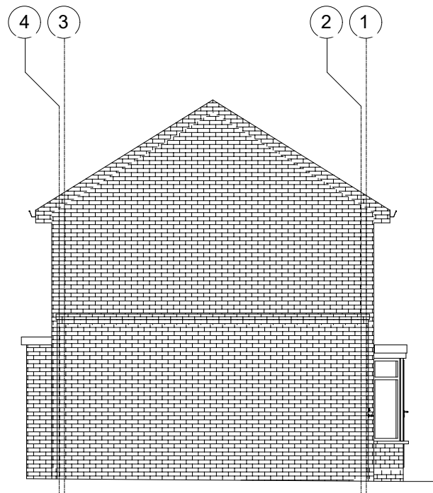
EXISTING RIGHT SIDE ELEVATION
