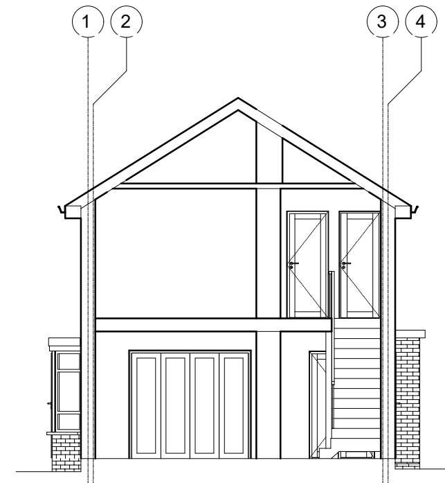
EXISTING SECTION
