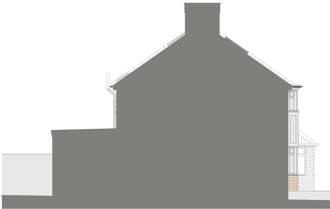
South-East Elevation 1:100
