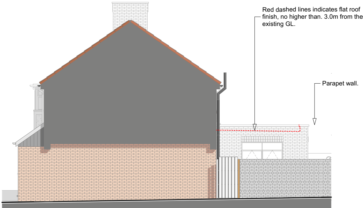
North-West Elevation 1:100
