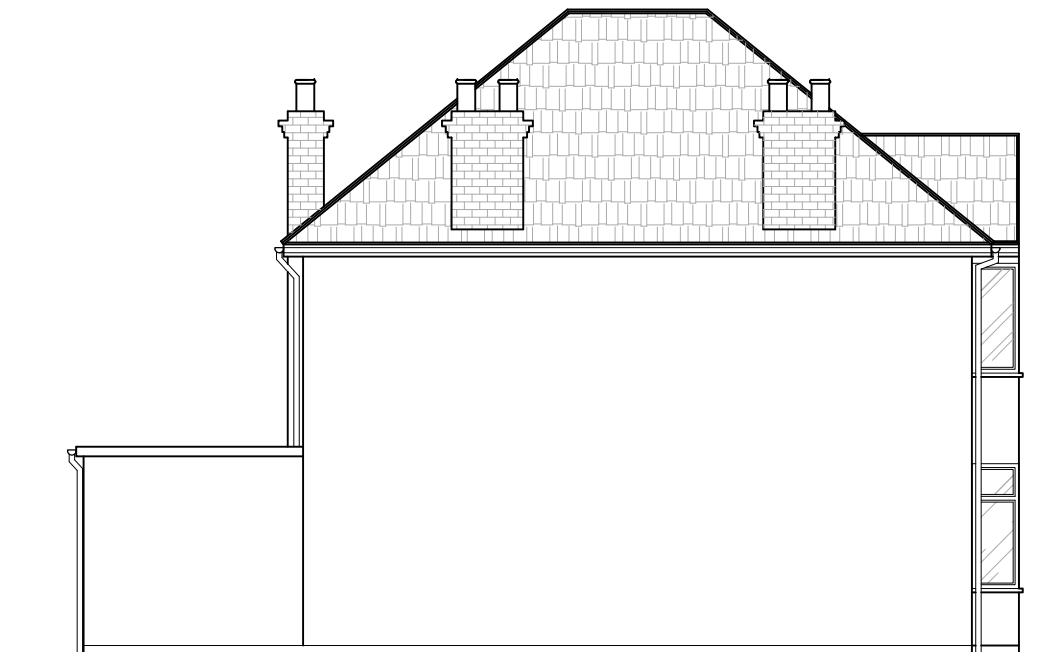
PROPOSED (LEFT) SIDE ELEVATION UN-CHANGED
