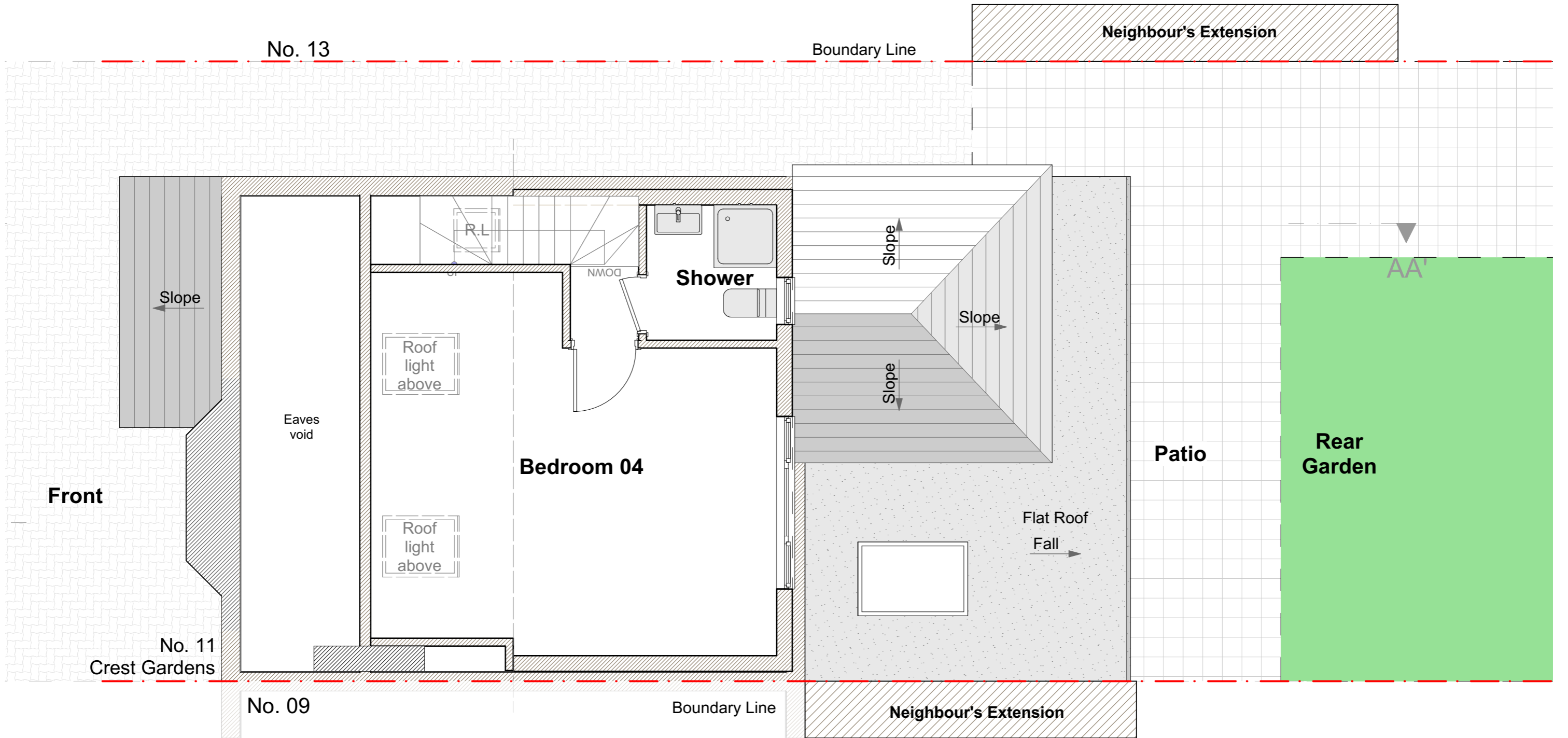
Proposed Second Floor Plan 1:50
