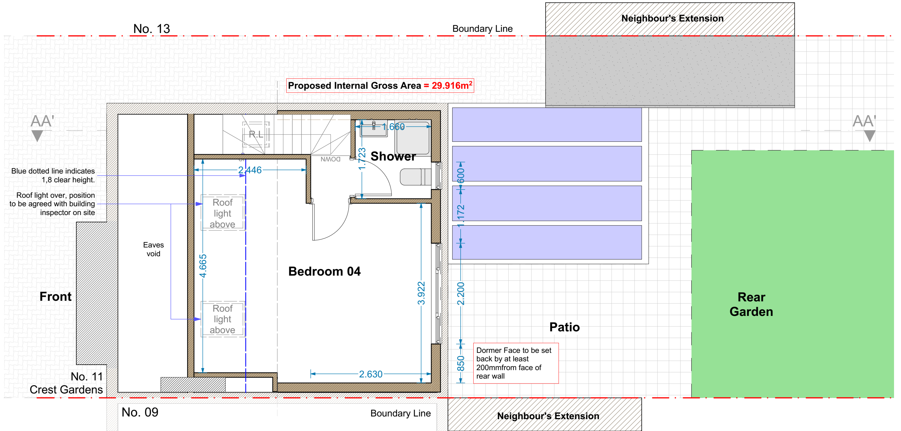
Proposed Second Floor Plan 1:50
