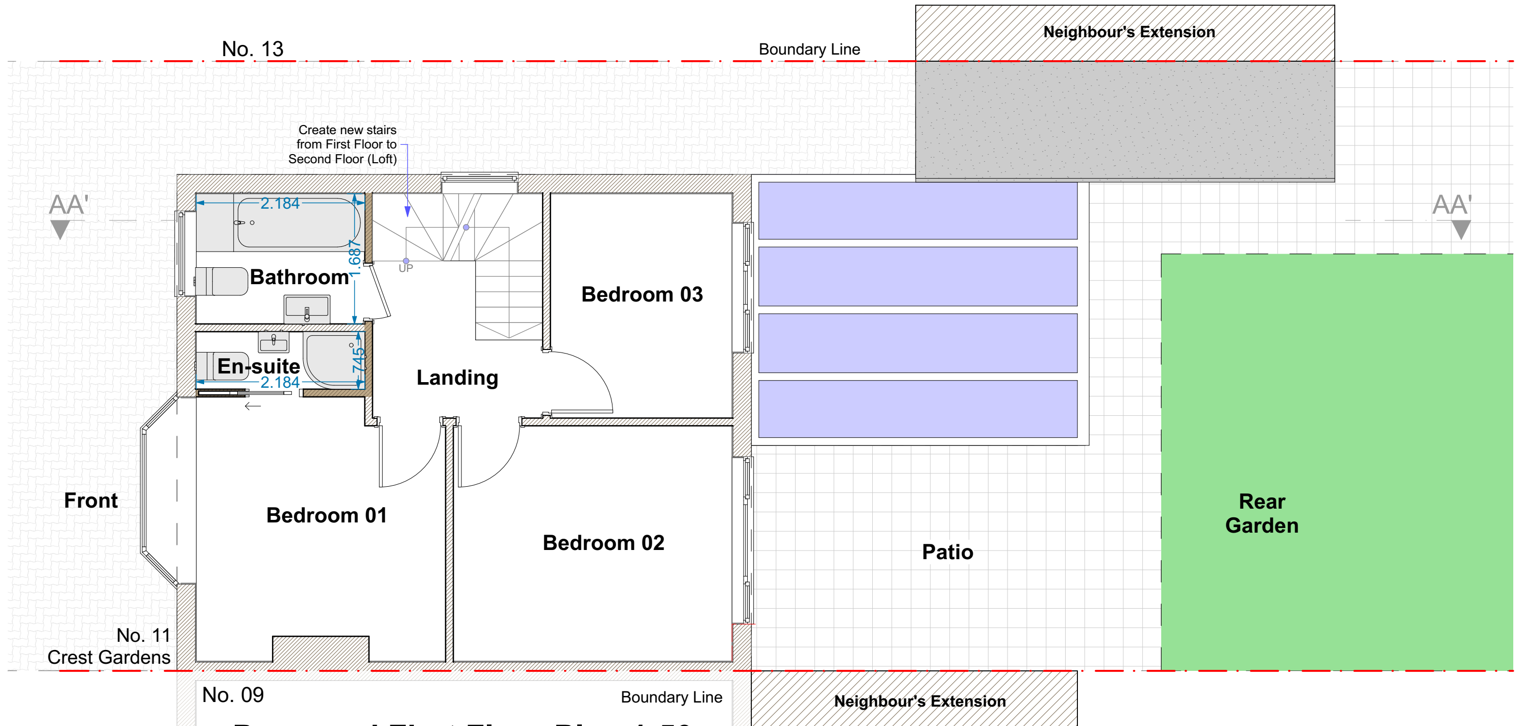
Proposed First Floor Plan 1:50
