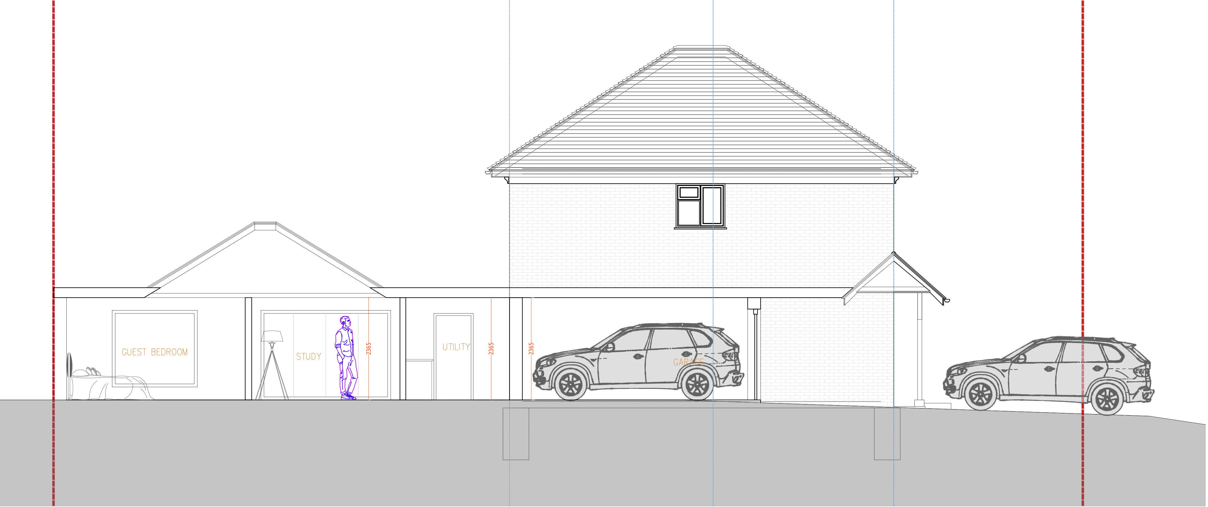
1 PR SECTION BB
