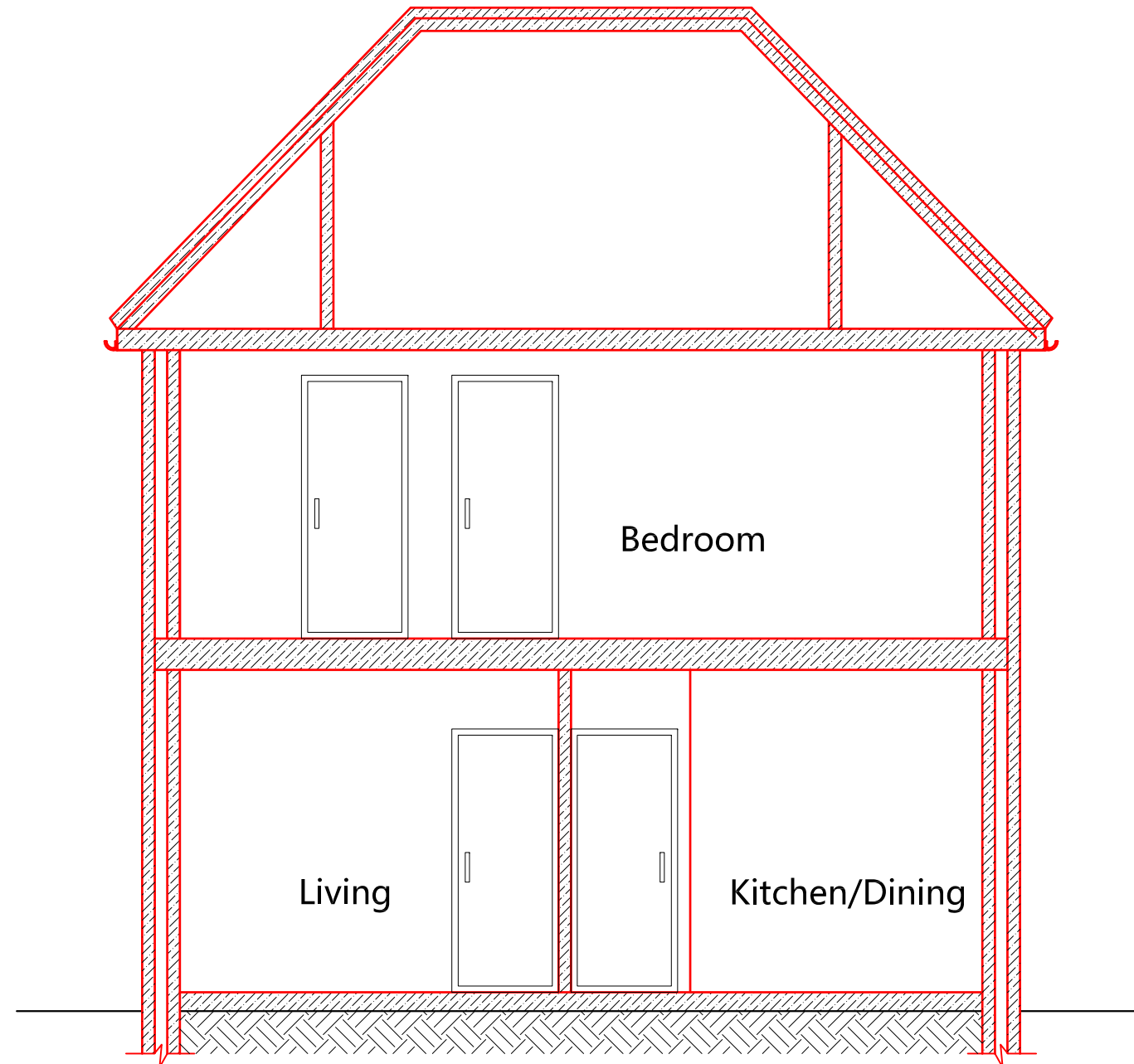
Section X-X
