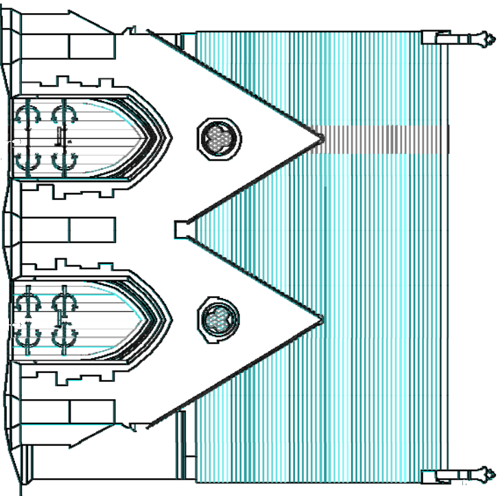
WEST ELEVATION
