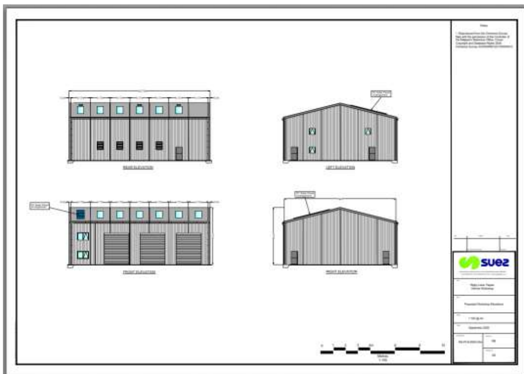
Figure 4: Proposed Elevations
