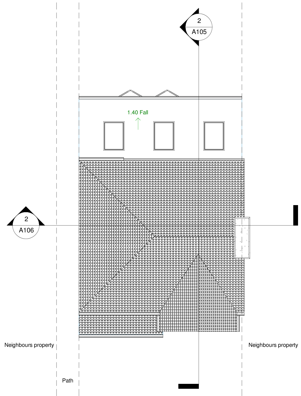
2 Roof - Proposed 1 : 100
