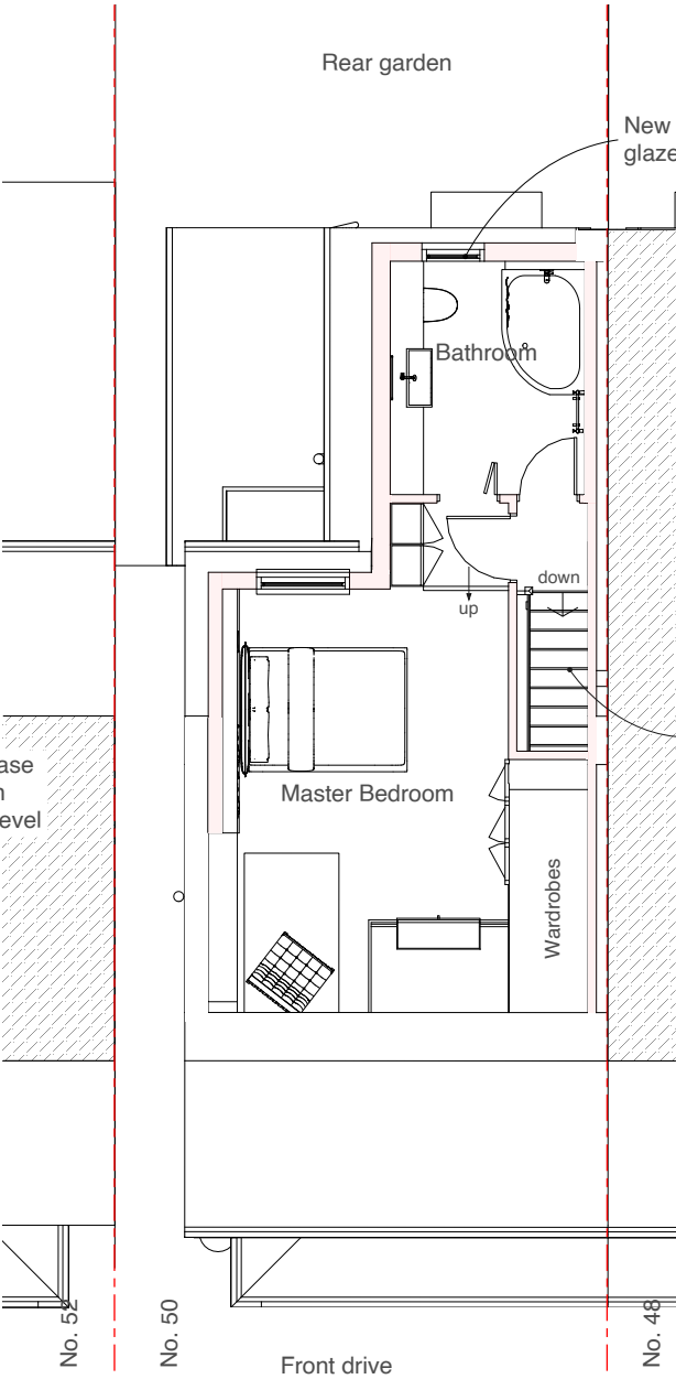
Proposed Loft Floor
