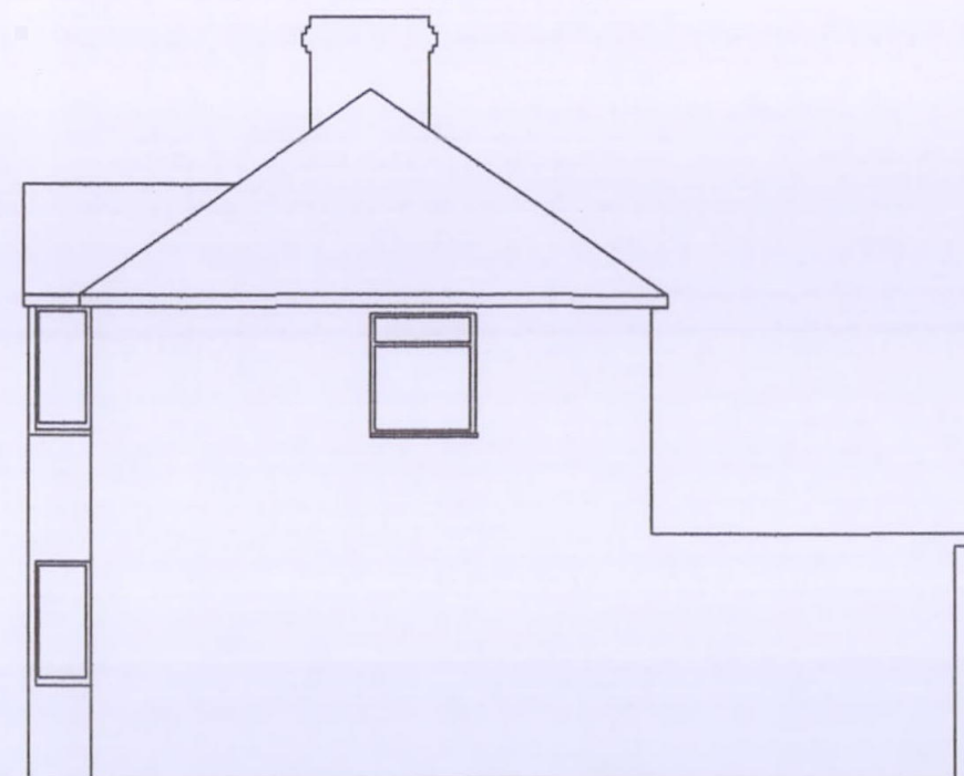
EXISTING WEST SIDE ELEVATION
