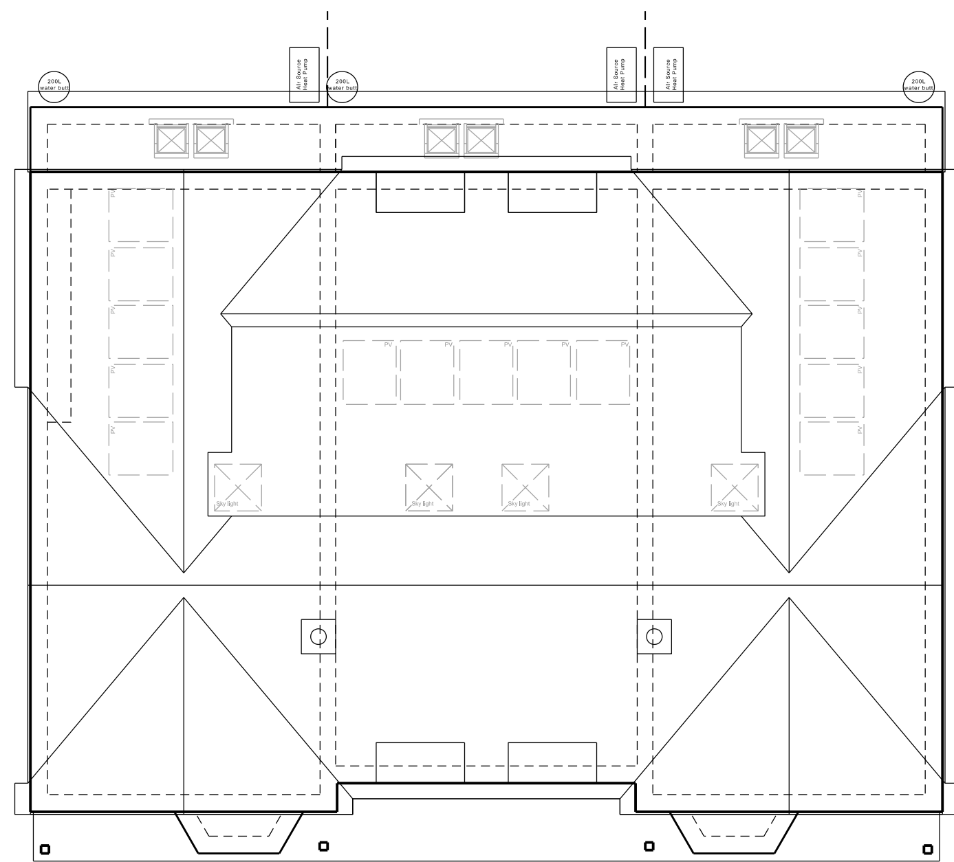
ROOF PLAN
