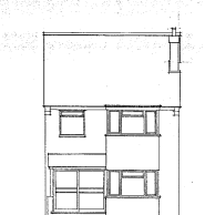
FRONT ELEVATION
