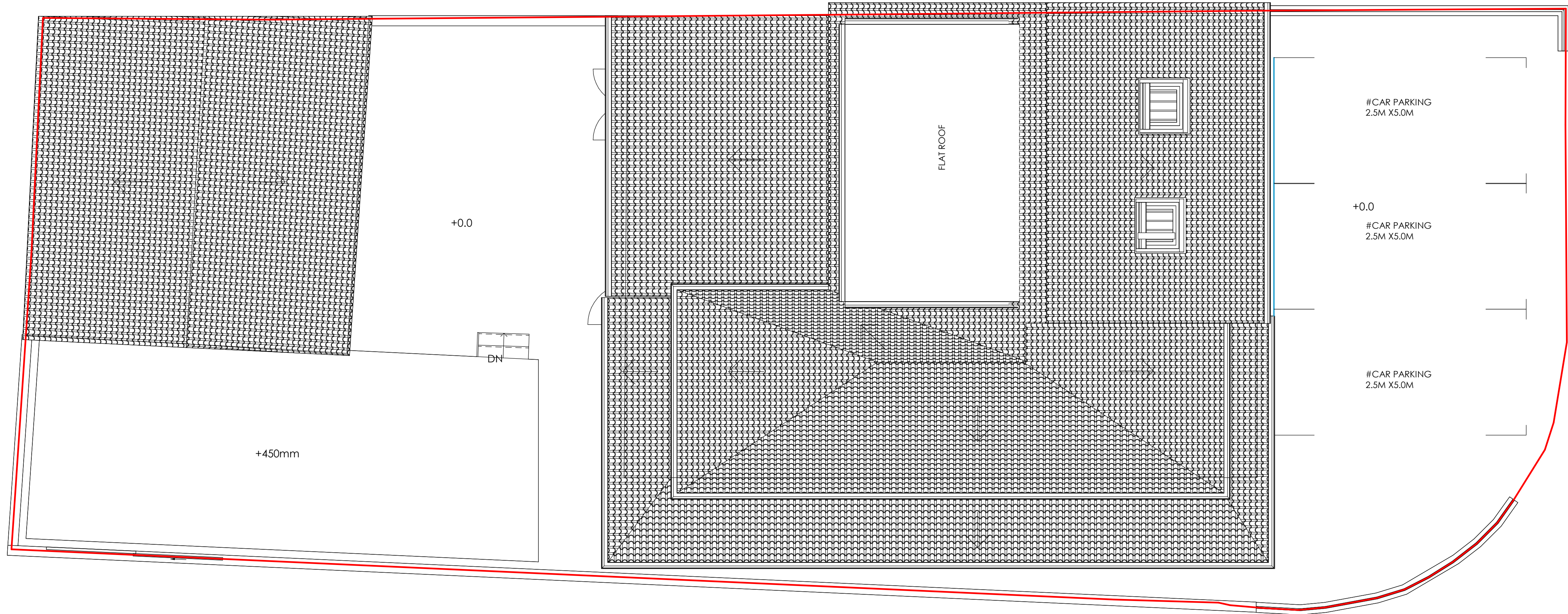
Proposed Roof Layout 1 : 50
