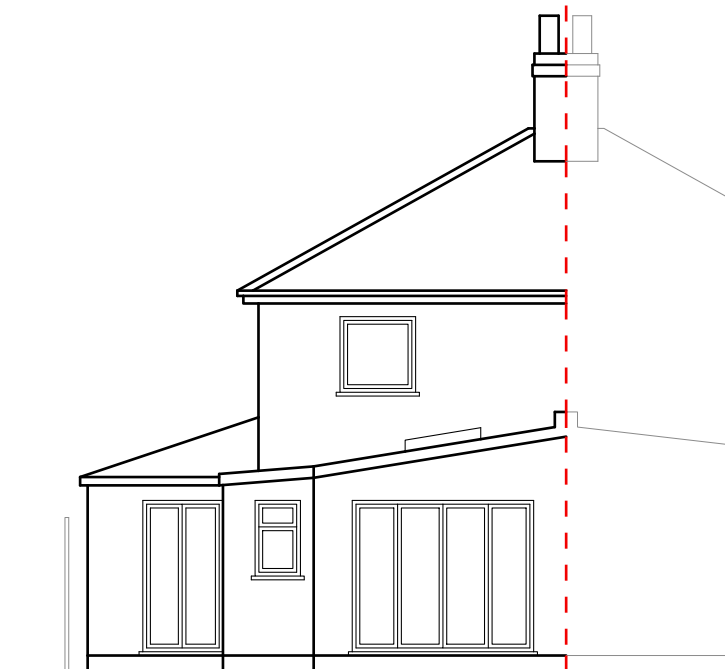
REAR ELEVATION
