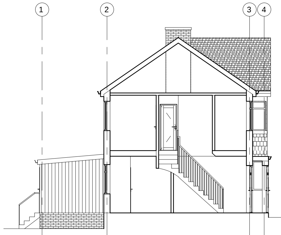
EXISTING SECTION
