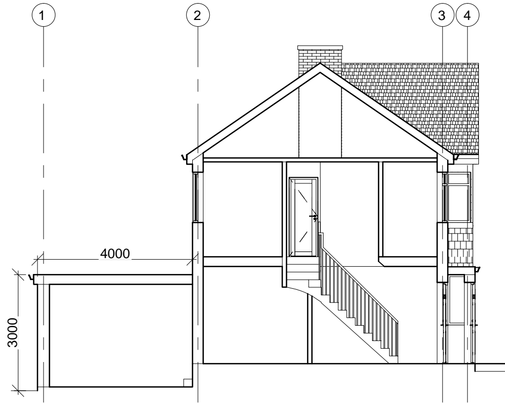
PROPOSED SECTION
