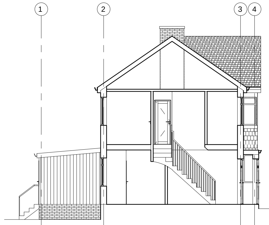
EXISTING SECTION
