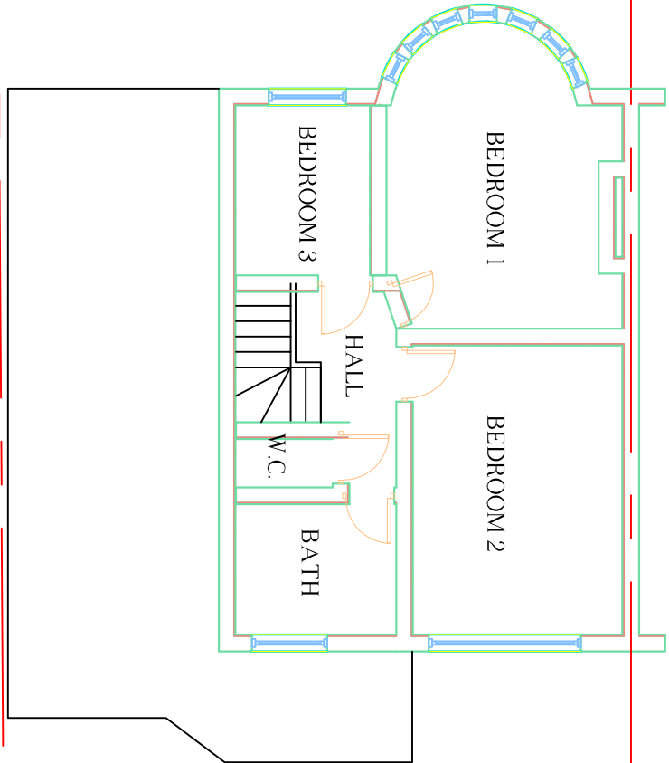
PRE-EXISTING FIRST FLOOR
