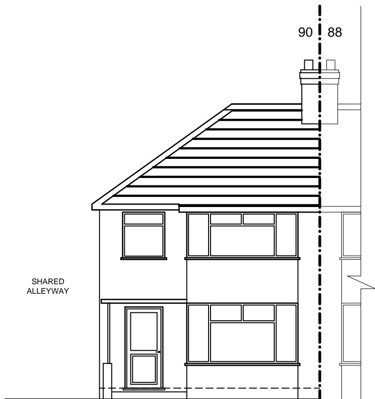
FRONT ELEVATION EXISTING
