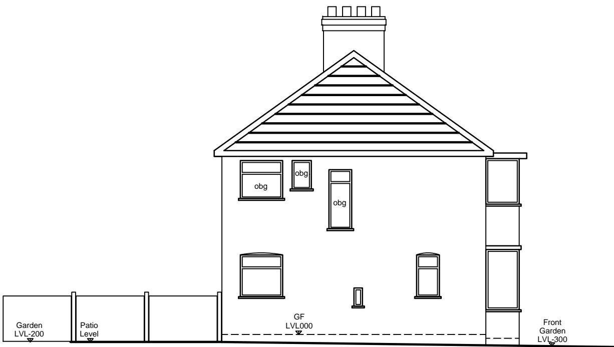
SIDE ELEVATION EXISTING (AS SEEN FROM SHARED ALLEYWAY)
