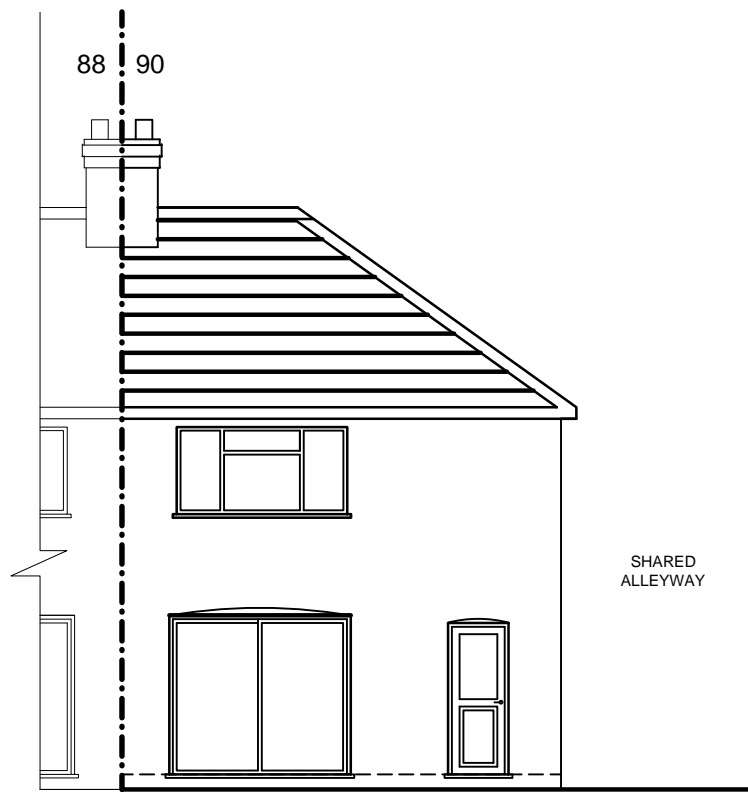
REAR ELEVATION EXISTING
