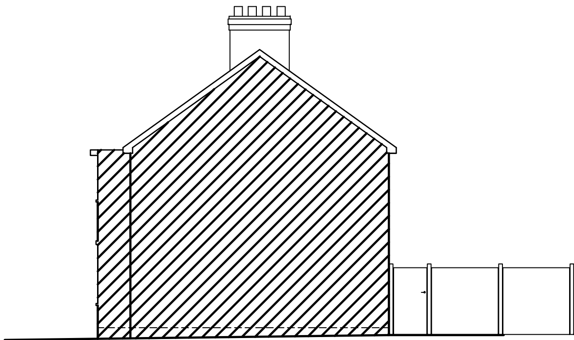
SIDE ELEVATION EXISTING (AS SEEN FROM NO.88)
