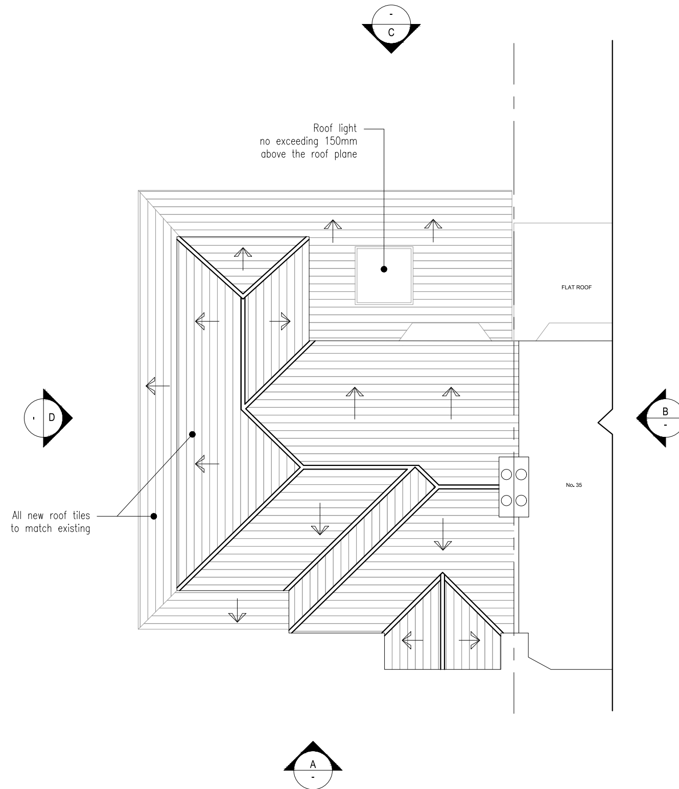
PROPOSED ROOF PLAN SCALE 1:100
