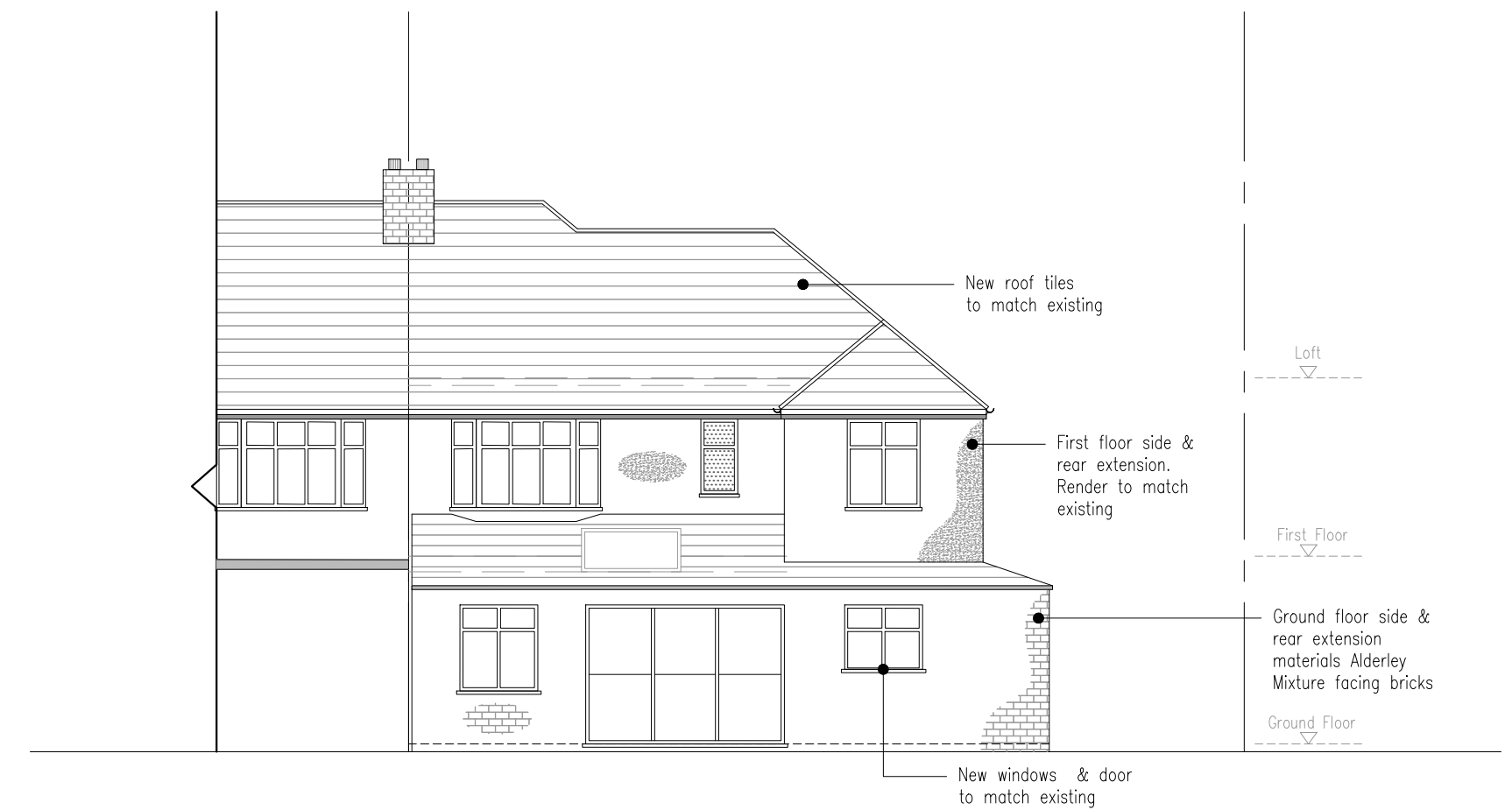
— PROPOSED REAR ELEVATION — C SCALE 1:100
