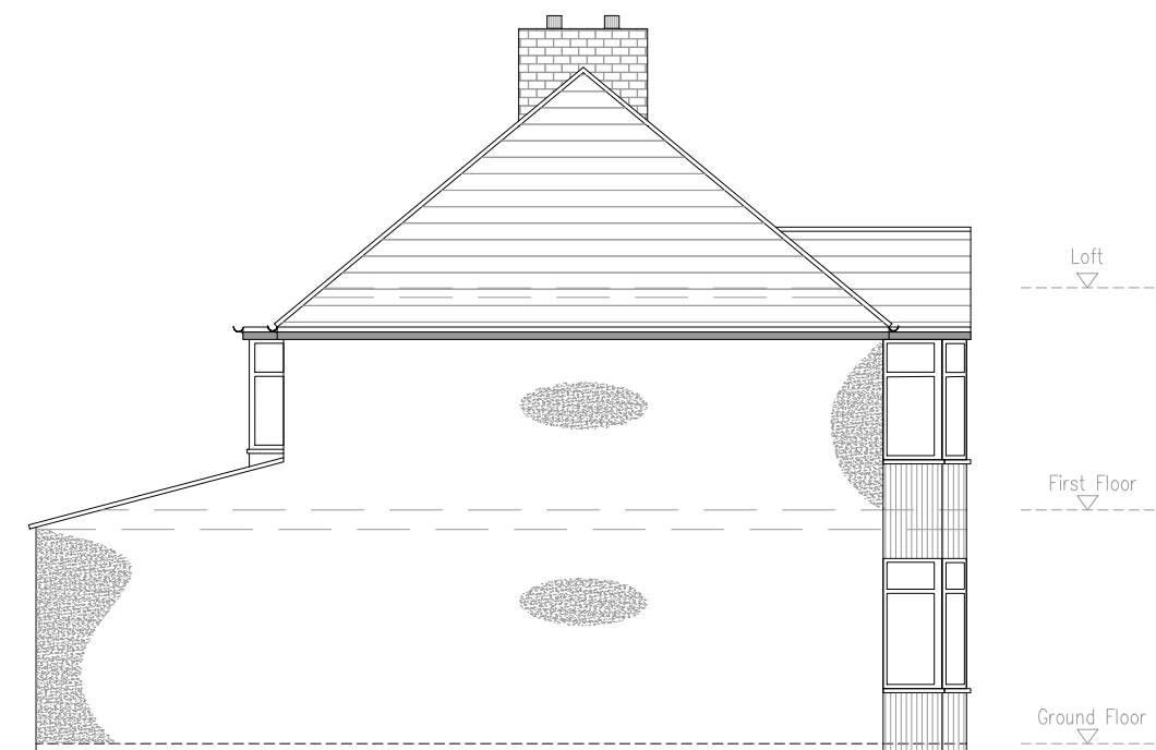
— EXISTING SIDE ELEVATION — D SCALE 1:100
