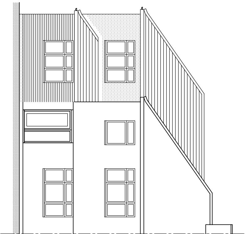
east elevation
