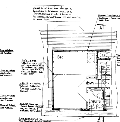
PROPOSED ROOMS IN LOFT SPACE
